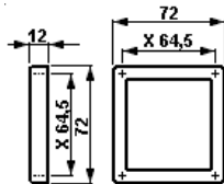
Glass for measuring instrument AM/VM72
