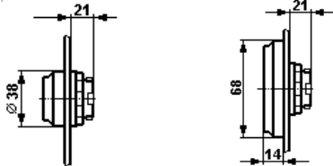
Bouton-poussoir double
