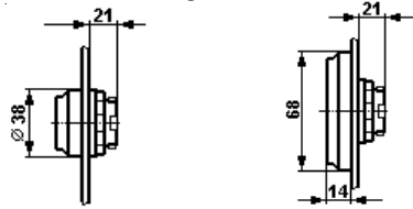
Push button
