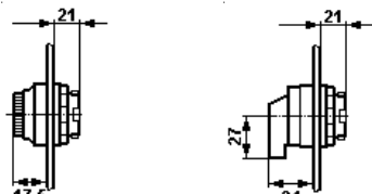
Signal lamp
