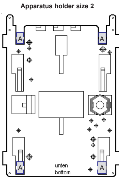
A = fixing point for control switches D22 292
