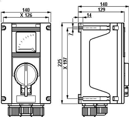
Control switch D22 293, with mes. instrument with direct connection
