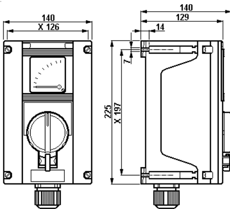
Control switch D22 293, with meas. instrument with c.t. connection
