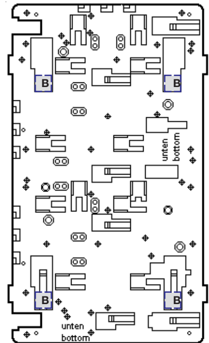
B = fixing point for control switches D22 293
