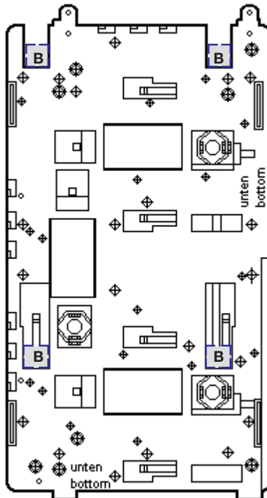
B = fixing point for control switches D22 293
