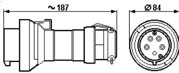
Plug 5-pole, GHG 511
