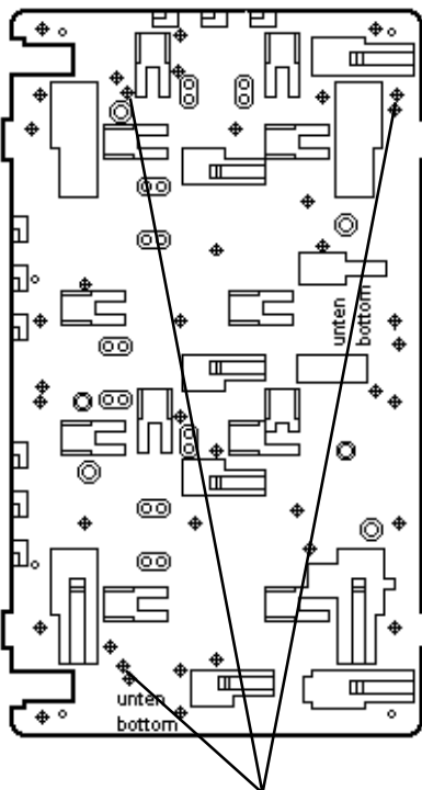
Apparatus holder for wall- and trellis fixing, size 3
