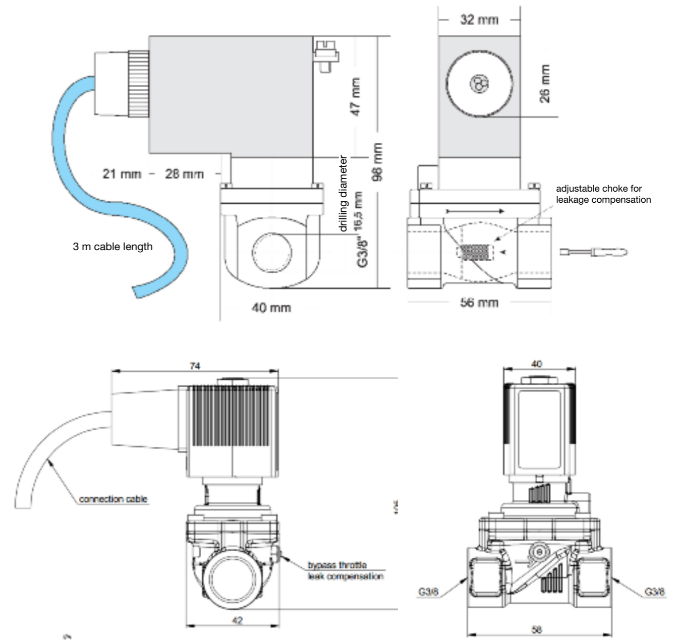
Figure 2: Solenoid valve SVD.L.x-Axx (top), SVD.L.x-Alxx (bottom)
