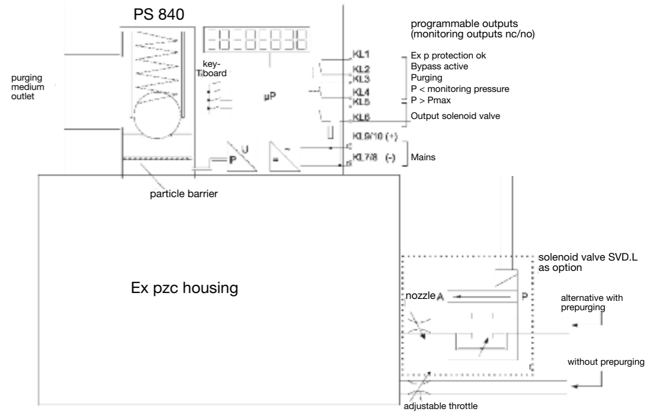
Figure 1 Block diagram
