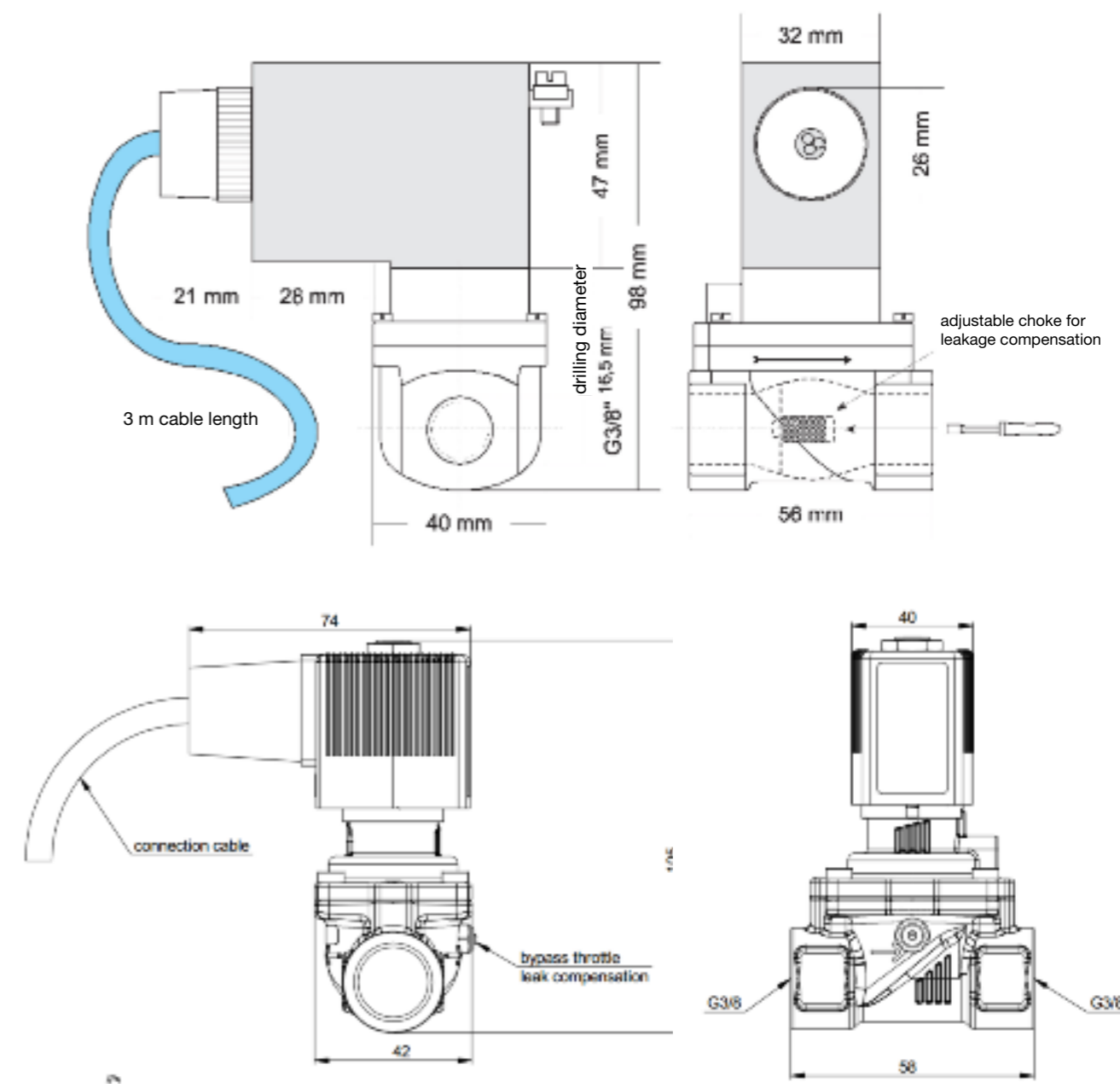
Figure 2: Solenoid valve SVD.L.x-Axx (top), SVD.L.x-Alxx (button)
