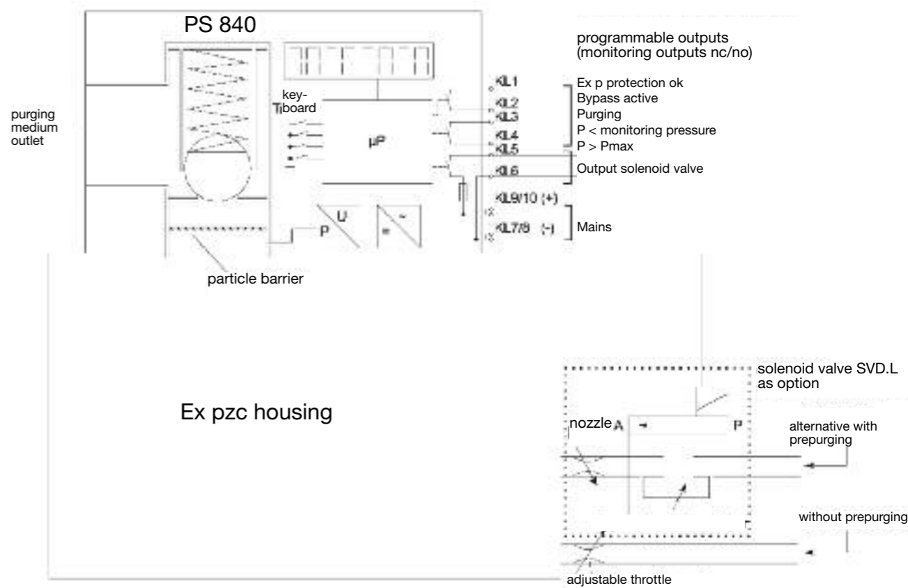
Figure 1 Block diagram
